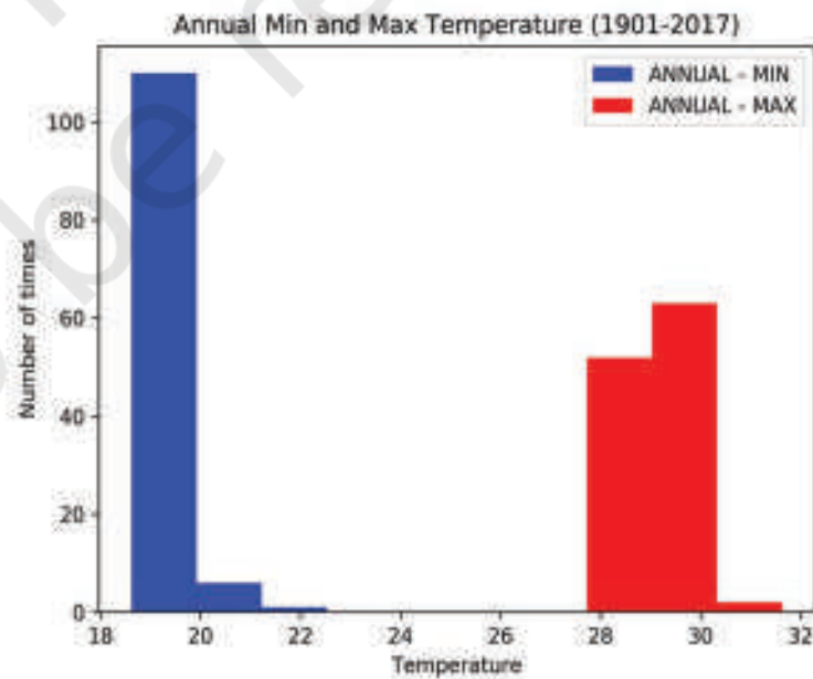
Figure 4.12: Histogram for 'ANNUAL - MIN'
